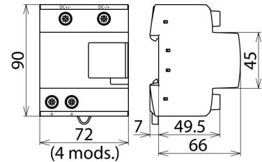
Dimension drawing DCB YPV 1500
